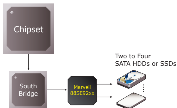
Fig 2. RAID-On-Motherboard Application
