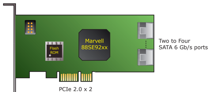
Fig 3. SATA RAID HBA Application
